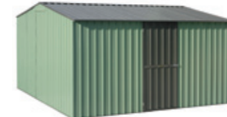
GM3838 3770 (w) x 3770 (d) x 1830 (h-min) mm Area: 14.21m 2 Height in centre: 2155mm
